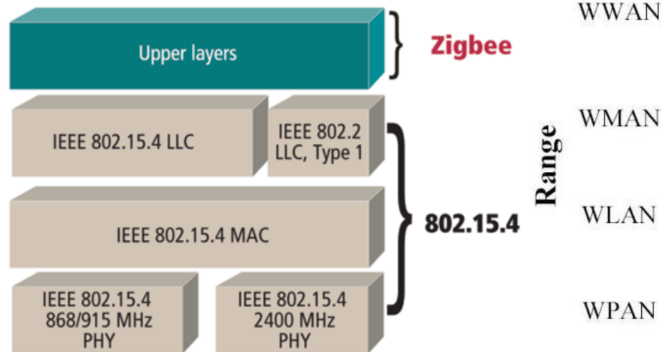
802.15.4 architecture
