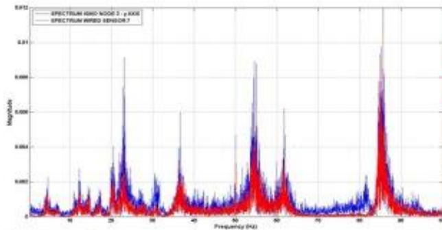
Vibrations-based Monitoring
