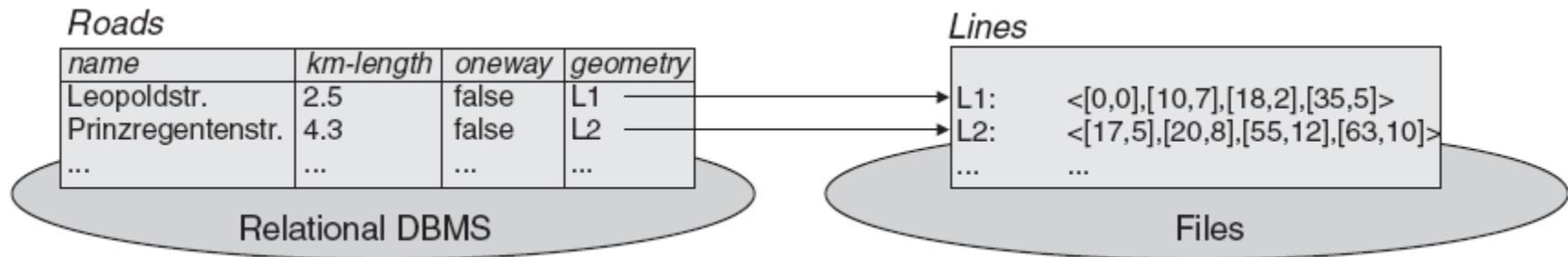
Loosely coupled
